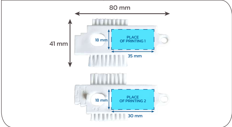
Dimensions/print area
